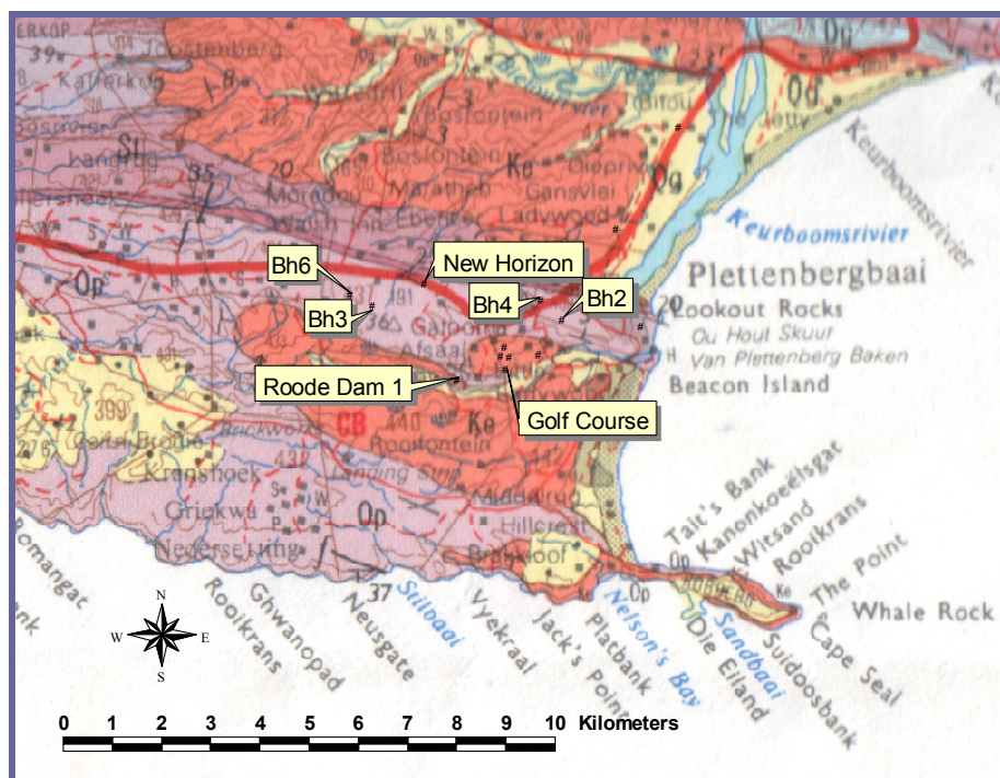
Op = Peninsula Formation orthoquartzites; Ke = Enon Formation conglomerates; St = Cedarberg Formation shales; Tc = Tchoando Formation sandstones; Qg = Unconsolidated gravel and sand (Source: 1: 250 000 Geological Map)
