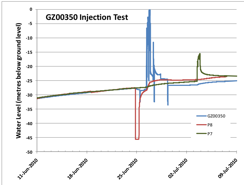
FIGURE 2.15 WATER LEVEL RESPONSE TO INJECTION OF 610 M 3 IN GZ00350
